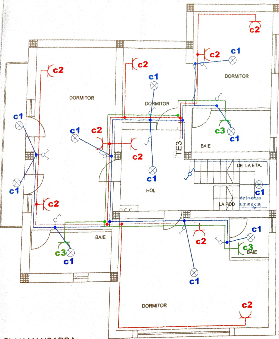
PLAN MANSARDA
